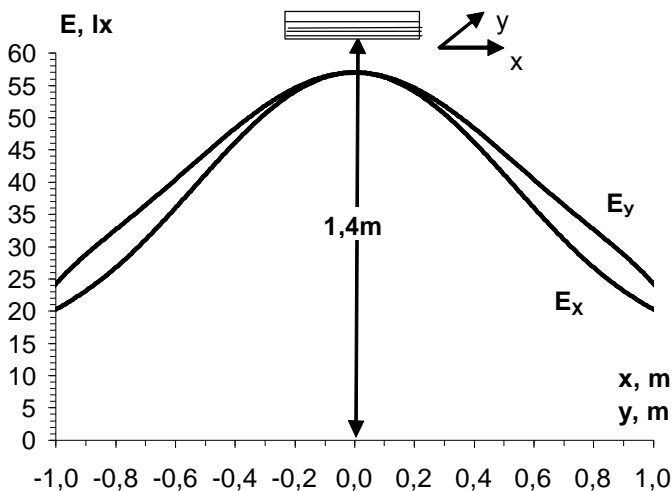
Longitudinal E_x and lateral E_y distribution of illuminance P=15 W.
