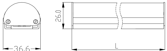
Outline drawing (in mm)
